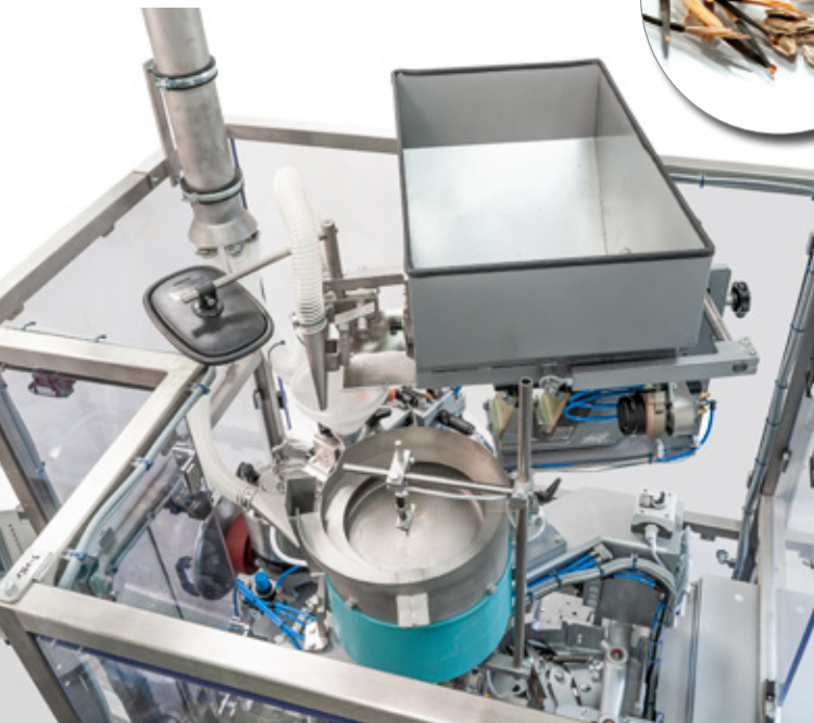
RTV bowl feeder dosing unit
