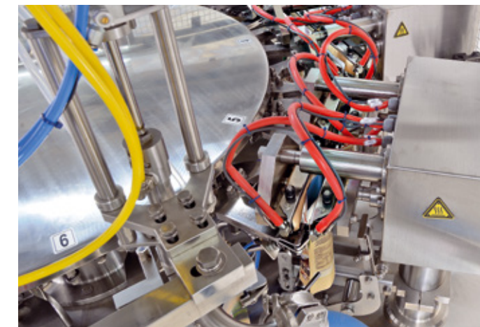
Double sealing and cooling of the top seam
